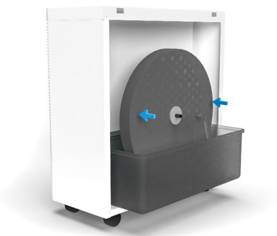
Fig. 4.2.7: Inserting the evaporative filter disc and water tank into the unit
